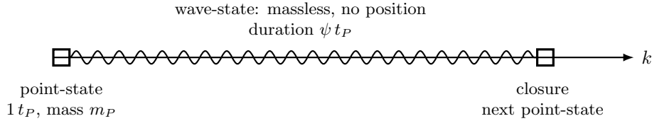
Figure 7: One branch cycle. The electron occupies a point-state for a single Planck tick and a wave-state for \psi ticks. The duty fraction 1/\psi = 4.18 \times 10^{-23} is what is observed as the electron’s mass ratio.
